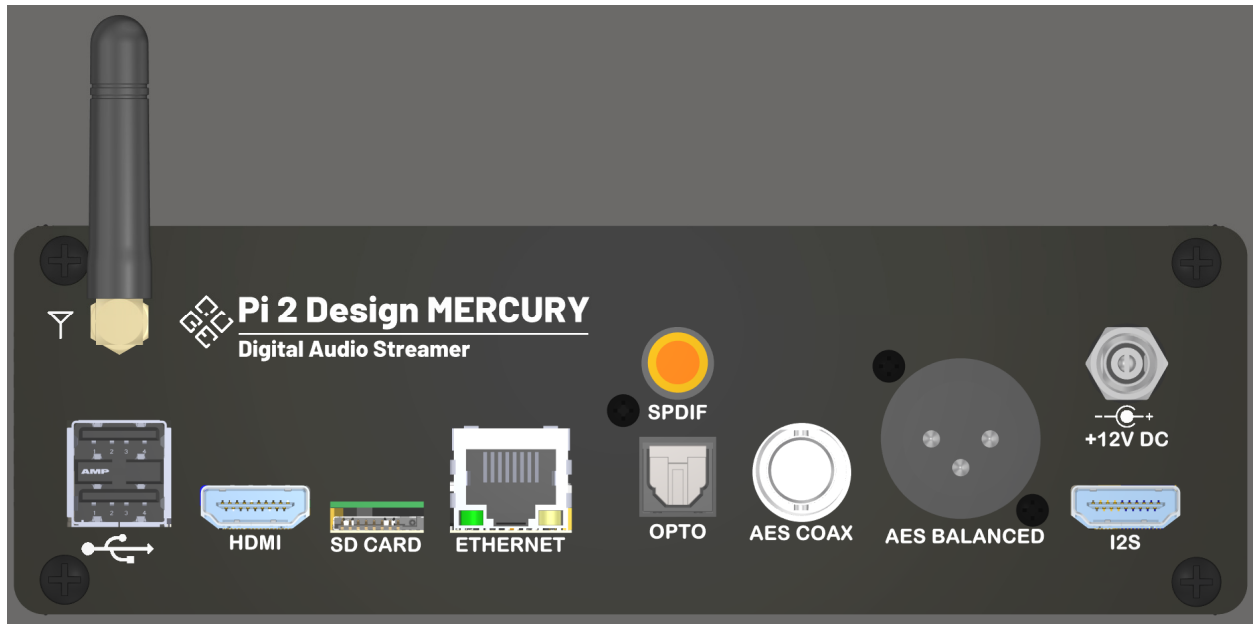
Figure 5 – Mercury Streamer Rear Panel
